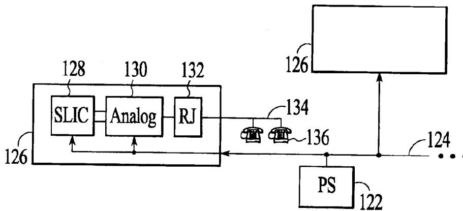
FIG. 7 (PRIOR ART)
